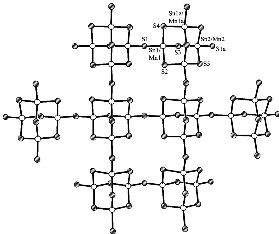
Fig. 27. Structure of \text{K}_2\text{MnSnS}_4 [7,134] in which the adamantane-like [\text{Mn}_2\text{Sn}_2\text{S}_{10}]^{6-} units are linked into sheets via common terminal S atoms.
