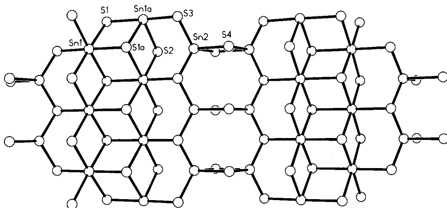
Fig. 10. Structure of the ^1_2[\text{Sn}_3\text{S}_7]^{2-} double chains in \text{K}_2\text{Sn}_3\text{S}_7 \cdot \text{H}_2\text{O} [10,121] and \text{Rb}_2\text{Sn}_3\text{S}_7 \cdot 2\text{H}_2\text{O} [104].
