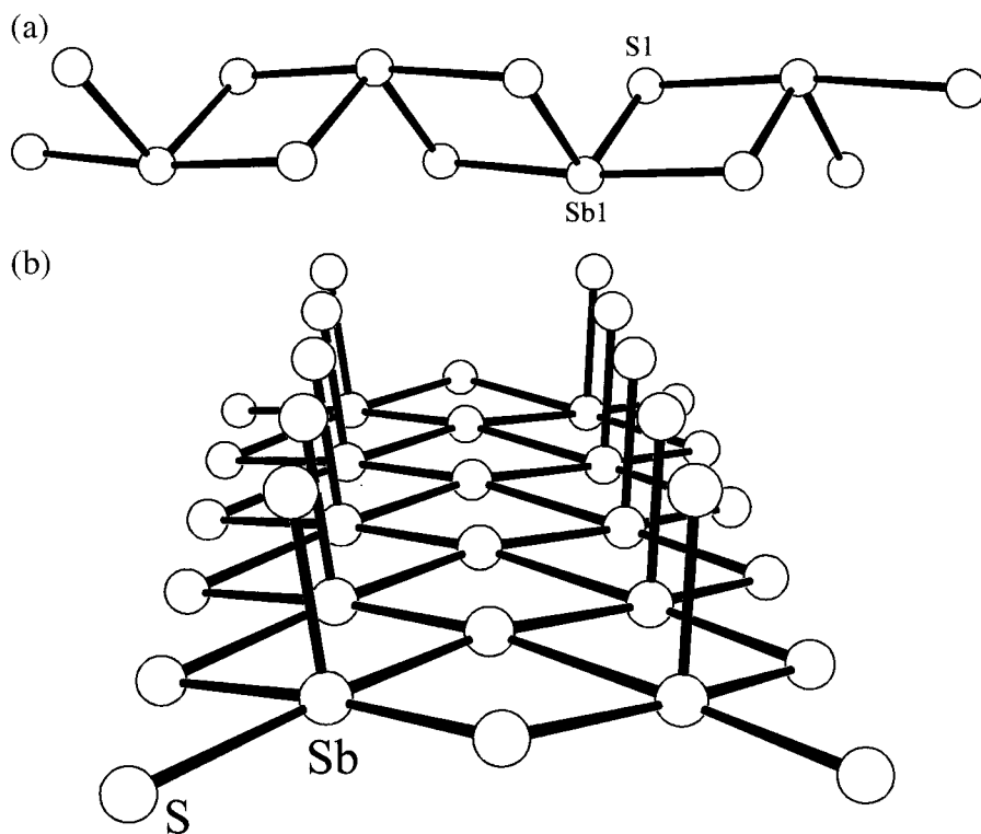
Fig. 38. (a) {}^1_2[\text{SbS}_2]^- chains with \psi -trigonal bipyramidal Sb atoms in \text{KSbS}_2 [277]. (b) {}^1_2[\text{Sb}_2\text{S}_5]^{4-} chains with \psi -octahedral Sb atoms in \text{Sr}_3\text{Sb}_4\text{S}_9 [282].
