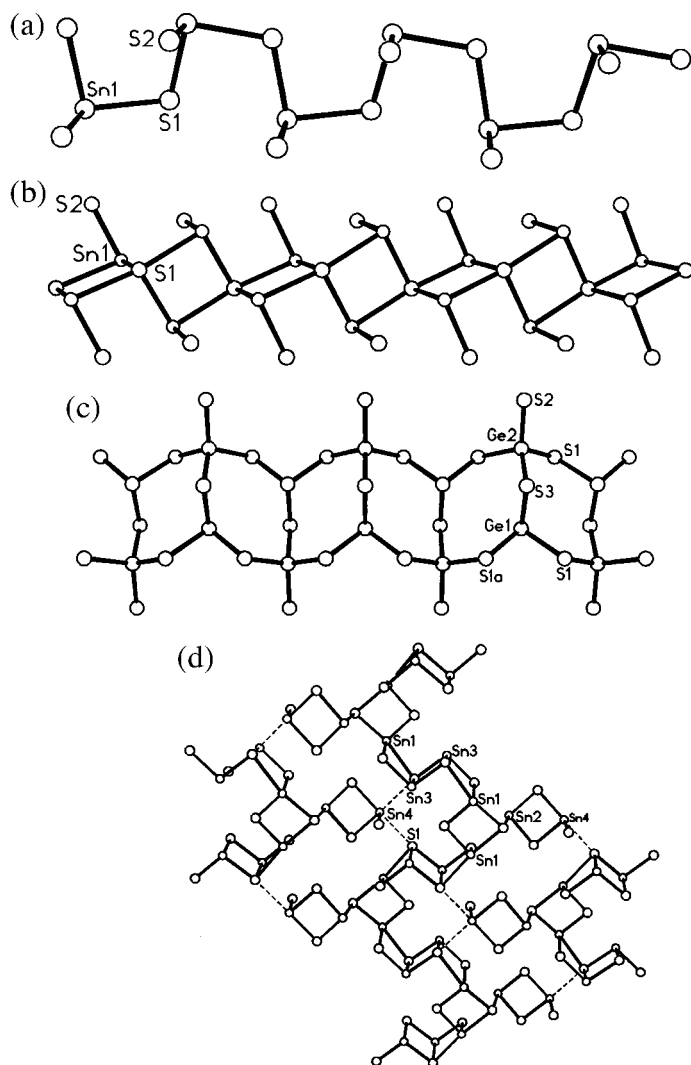
Fig. 33. (a) The chain structure {}_{\infty}[\text{SnS}_2]^{n-1} of \text{BaSnS}_2 [35], (b) connection of two such chains through common bridging S atoms in \text{Tl}_2\text{Sn}_2\text{S}_3 [226], which possess \psi -trigonal bipyramidal environments, (c) two Ge-S ribbons with alternating \text{Ge}^{\text{II}} / \text{Ge}^{\text{IV}} positions, that are linked into a double chain by additional \text{Ge}^{\text{II}}-\text{S} bonds in \text{Tl}_2\text{Ge}_2\text{S}_4 [28] and (d) the {}_{\infty}[\text{Sn}_2\text{S}_2]^{n-2} sheet anion in \text{BaSn}_2\text{S}_3 [36] with \text{Sn4} \cdots \text{S1} interactions of 3.269(7) Å depicted as dashed lines.
