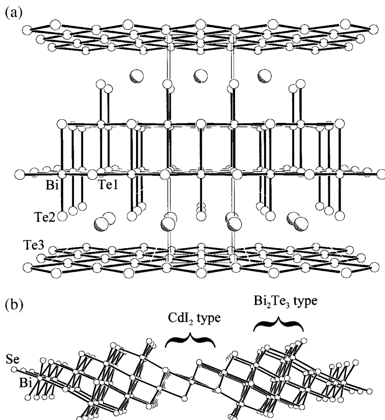
Fig. 53. (a) Structure of \text{SrBiTe}_3 and isostructural \text{SrSbTe}_3 [366,367] with alternating ^{2-}[\text{Bi}(\text{Sb})\text{Te}_2] and ^{2-}[\text{Te}_3] sheets; (b) sheets consisting of \text{Bi}_2\text{Te}_3 - and \text{CdI}_2 -type fragments in \text{Cs}_3\text{Bi}_7\text{Se}_{12} [327]; similar sheets occur in \text{Sr}_4\text{Bi}_6\text{Se}_{13} [324].
