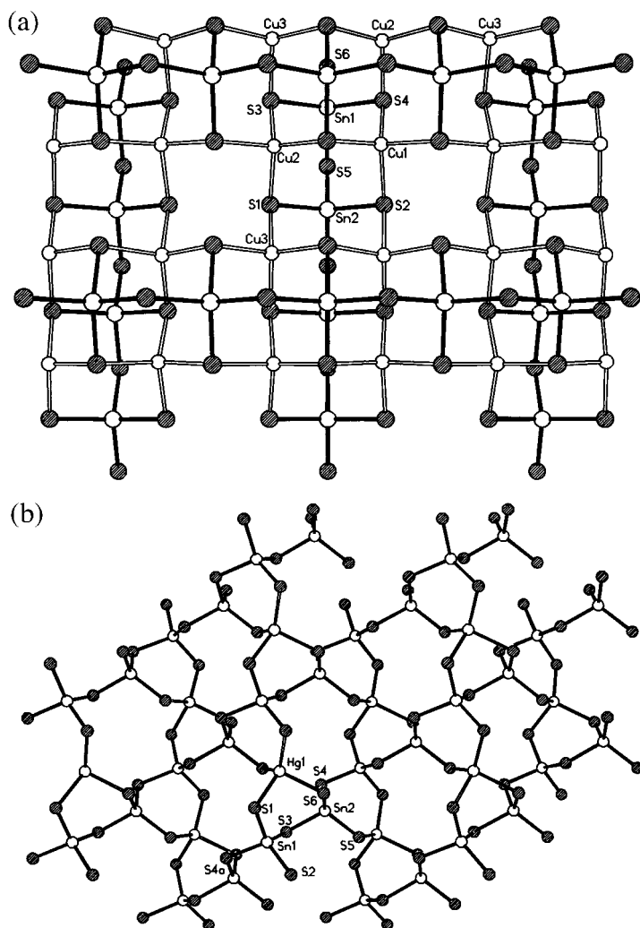
Fig. 26. The sheets (a) of the isostructural compounds ACuSnE_3 ( A = Na, K, Rb, Cs ; E = S : A = K, Rb ; E = Se ) [213] and (b) of K_2HgSn_2S_6 [7,134]. All compounds display ^1_2[SnS_3]^{2-} chains [16,17,115–120] as structure building components.
