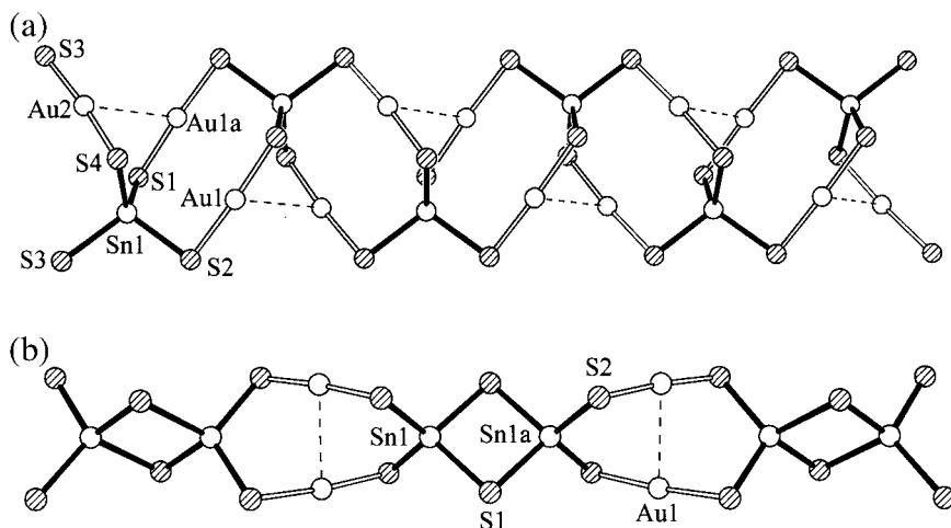
Fig. 28. The chain structures of the potassium phases (a) K_2Au_2SnS_4 and (b) K_2Au_2Sn_2S_6 [213]. The Au^I atoms in both compounds exhibit linear S–Au–S coordination and short Au \cdots Au contacts of 3.363(2) and 3.010(2) Å, respectively.
