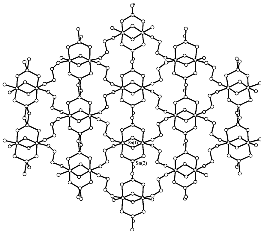
Fig. 17. The sheet structure of the {}^2_z[\text{Sn}_2\text{S}_8]^{2-} anion in \text{K}_2\text{Sn}_2\text{S}_8 [151].
