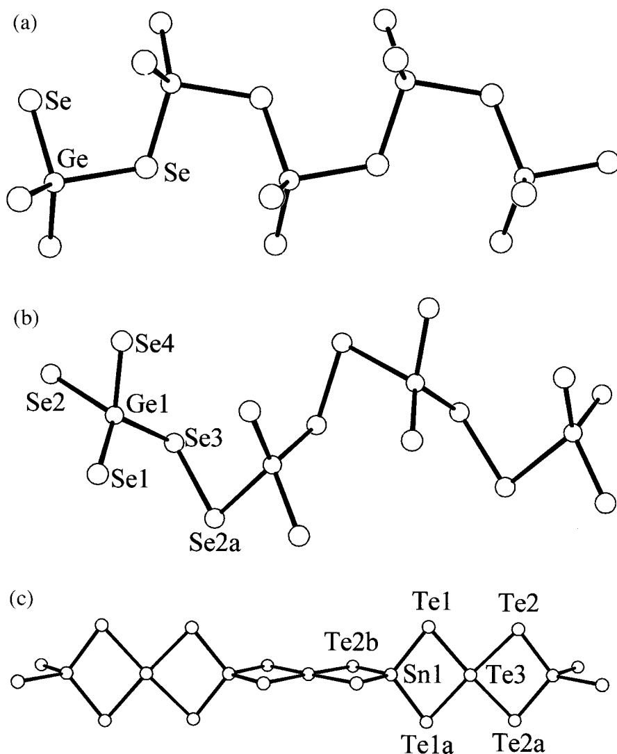
Fig. 8. Polymeric chainlike anions with mononuclear \text{ME}_4 ( \text{M} = \text{Sn}, \text{Ge} ) building units in (a) ^{1/2}[\text{GeSe}_3]^{2-} in \text{Na}_2\text{GeSe}_3 [88], (b) ^{1/2}[\text{GeSe}_4]^{2-} in \text{K}_2\text{GeSe}_4 [83] and (c) ^{1/2}[\text{SnTe}_5]^{2-} in \text{K}_2\text{SnTe}_5 [135].
