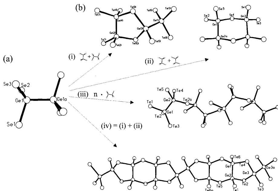
Fig. 36. (a) The dinuclear M(III) anion [M_2E_6]^{6-} in compounds A_6M_2E_6 ( A = Na, K, Rb, Cs, Tl ; M = Si, Ge, Sn ; E = S, Se, Te ). (b) Condensation pathways to oligo- or chain chalcogenidometalates(III): (i) 'head to head and tail' condensation of two [M_2E_6]^{6-} units leading to the [M_4E_{10}]^{8-} anion (modification I) present in Na_8Si_4Te_{10} [234], Na_8Ge_4Se_{10} (I) [235] and Na_8Ge_4Te_{10} (I) [234]; (ii) the 'head to head/tail to tail' condensation of two [M_2E_6]^{6-} units that generates [M_4E_{10}]^{8-} as modification II in both Na_8Ge_4Se_{10} (II) [24] and Na_8Ge_4Te_{10} (II) [236]; (iii) corner-linking of Ge_2Te_6 -octahedra to the [Ge_2Te_5]^{4-} chain of Ba_2Ge_2Te_5 [26]; and (iv) combination of pathways (i) and (ii) to afford the {}_2[Ge_6Te_{12}]^{6-} anion in Li_6Ge_6Te_{12} [27].
