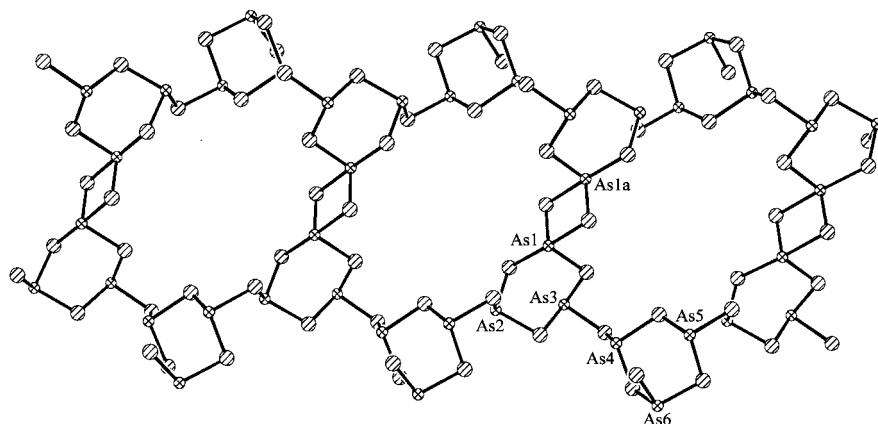
Fig. 1. \psi - \text{AsS}_4 trigonal bipyramidal coordination polyhedra in the {}^1_x[\text{As}_6\text{S}_{10}]^{2-} double chains of (\text{Me}_4\text{N})_2[\text{As}_6\text{S}_{10}] [51].
