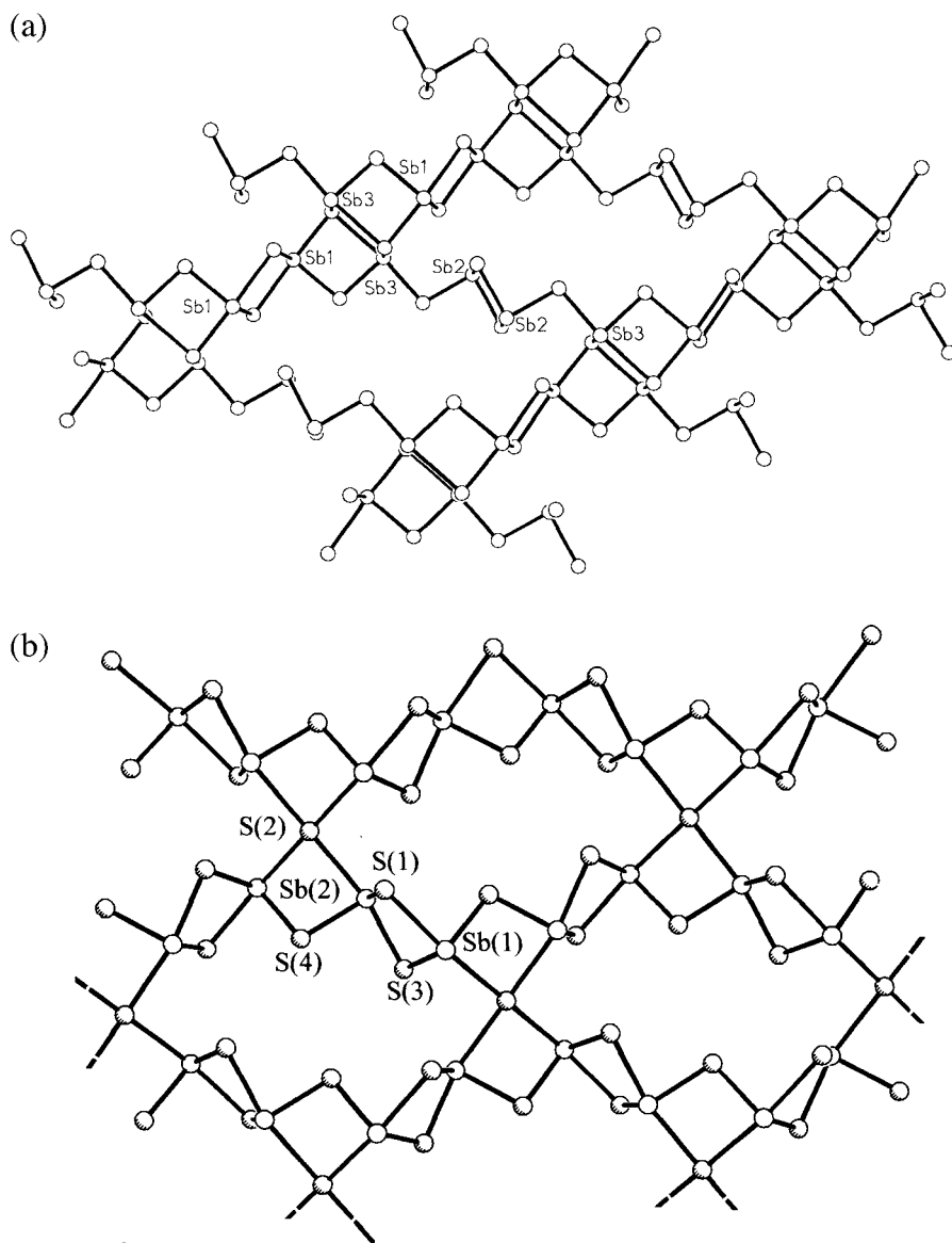
Fig. 49. Ribbons as structural motifs in lamellar thioantimonates: (a) cross-linked [\text{Sb}_4\text{S}_8]^{4-} chains in \text{RbSb}_3\text{S}_5 \cdot \text{H}_2\text{O} [296]; and (b) [\text{SbS}_2] chains with bridging \mu_4 -S atoms in \text{Rb}_2\text{Sb}_4\text{S}_7 [296].
