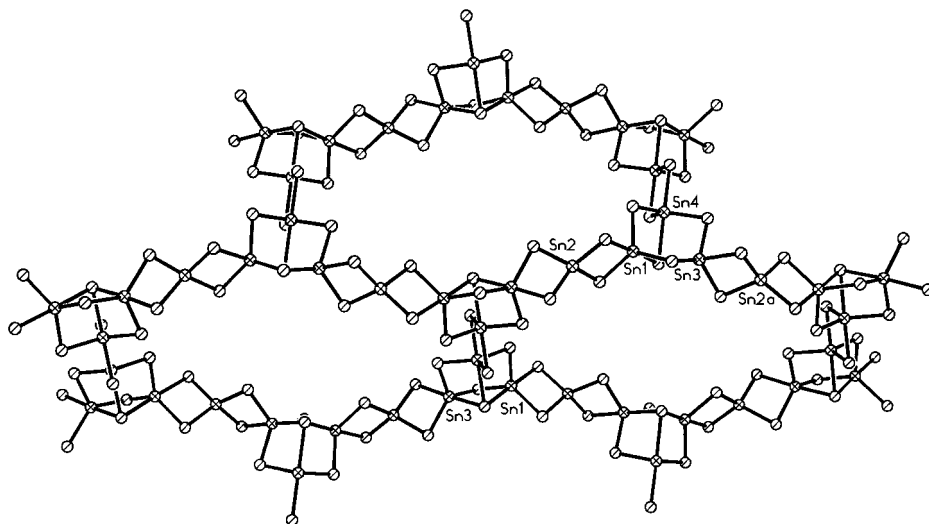
Fig. 14. Lamellar structure of the ^{2-}_2[\text{Sn}_4\text{S}_9]^{2-} anion in (\text{Bu}^n)_2\text{Sn}_4\text{S}_9 [127].
