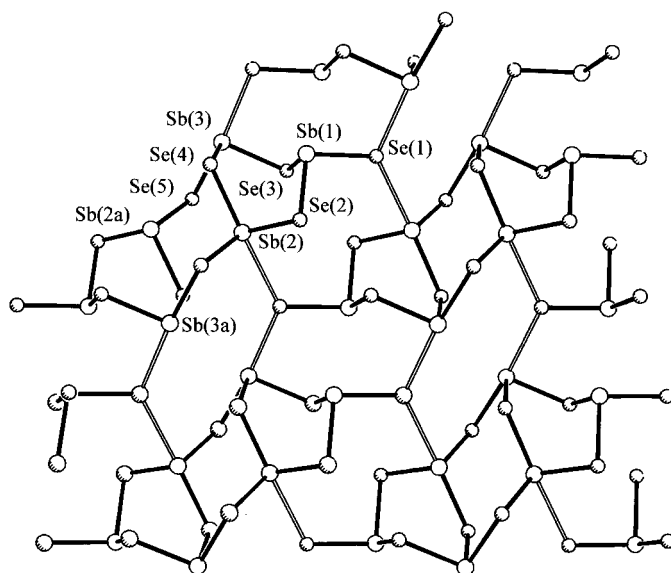
Fig. 2. The anion sheet {}^2[\text{Sb}_3\text{Se}_5]^- in \text{RbSb}_3\text{Se}_5 [57]. Sb–Se distances shorter than 2.73 Å are depicted as full bonds, the longer Sb(2)–Se(1) and Sb(3)–Se(1) interactions [3.055(2), 3.103(2) Å] as open bonds.
