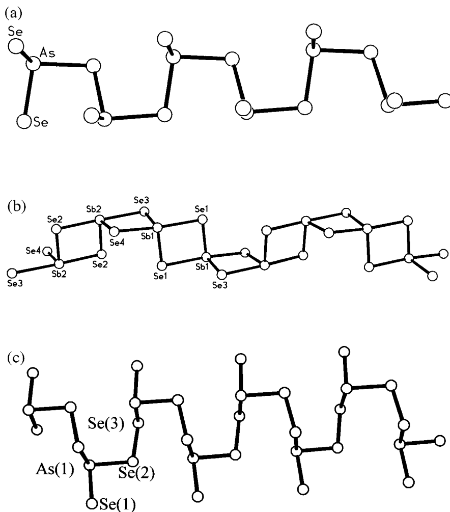
Fig. 43. Polymeric chain-like anions with mononuclear ME_3 or ME_4 building units ( M = As, Sb ): (a) \frac{1}{2}[AsSe_2^-] chains in NaAsSe_2 [261]; (b) \frac{1}{2}[SbSe_2^-] chains in KSbSe_2 [283]; (c) \frac{1}{2}[AsSe_3^-] chains in KAsSe_3 \cdot H_2O [263].
