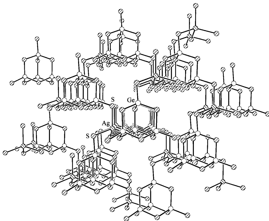
Fig. 22. Open zinc blende-like framework structure of {}^3_2[\text{AgGe}_4\text{Se}_{10}]^{3-} in \text{Rb}_3[\text{AgGe}_4\text{Se}_{10}] \cdot 2\text{H}_2\text{O} [192].
